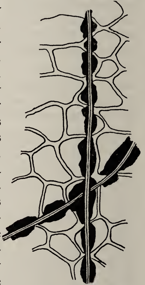
FIG. 8. Stylets and stylet tracks in bark parenchyma.
