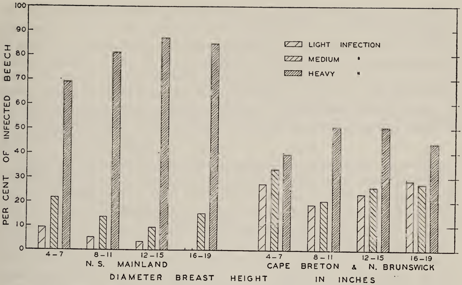
FIG. 13. Percentages of Nectria -infected beech with light, medium, and heavy infection, by diameter classes; in Nova Scotia mainland, and in New Brunswick and Cape Breton Island.
